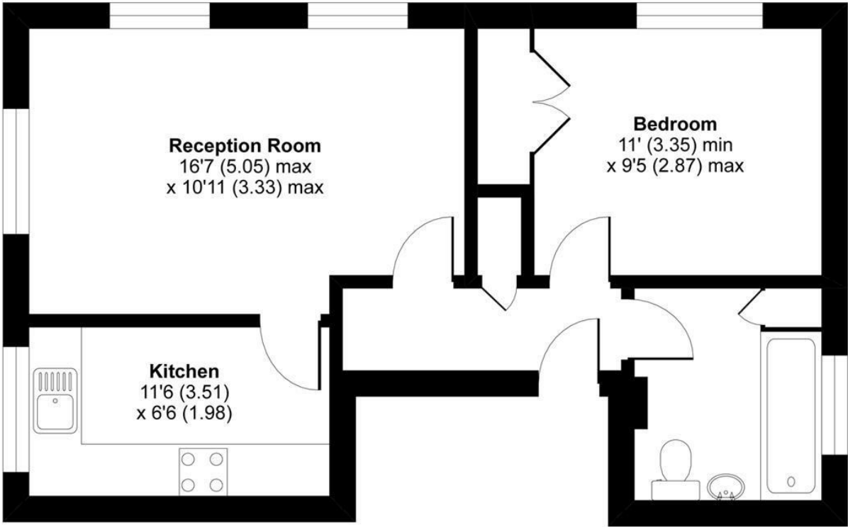
FIRST FLOOR
